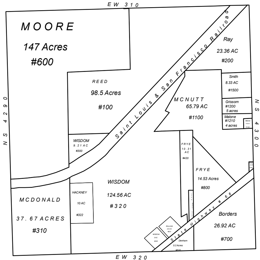
Section 14 Township 24N Range 18E
